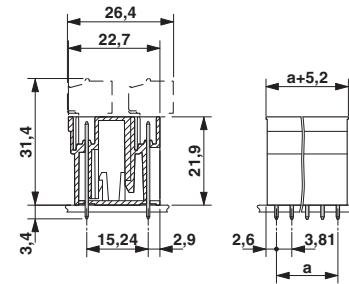
Dimensional drawing
