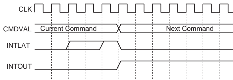
Figure 4-7 • Interrupt Vector Extender Timing
