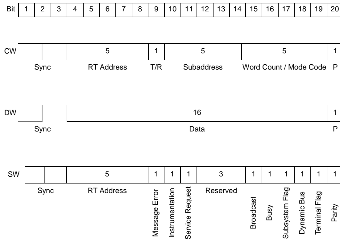
Figure 1-2 • 1553B Word Formats
