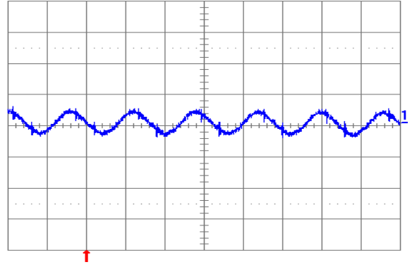
Fig. 3.3V.6: Output voltage ripple (20mV/div.) at full rated load current into a resistive load with external capacitance 100\mu F ceramic and V_{in} = 12V for V_{out} = 3.3V . Time scale: 2 \mu s /div.
