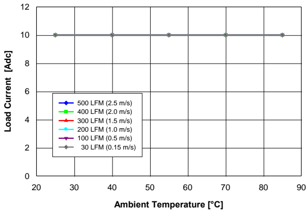
Fig. 1.5V.1: Available load current vs. ambient temperature and airflow rates for V_{out} = 1.5V converter mounted vertically with V_{in} = 12V , and maximum MOSFET temperature \leq 120^\circ C .
