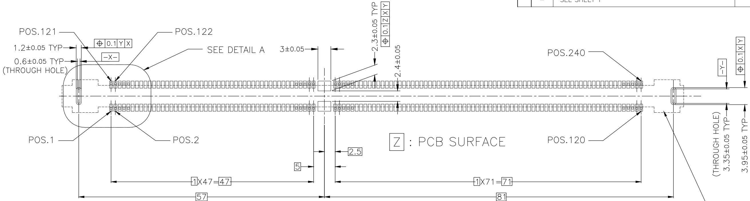
REFERENCE PCB LAYOUT (VIEWED FROM CONNECTOR SIDE)
