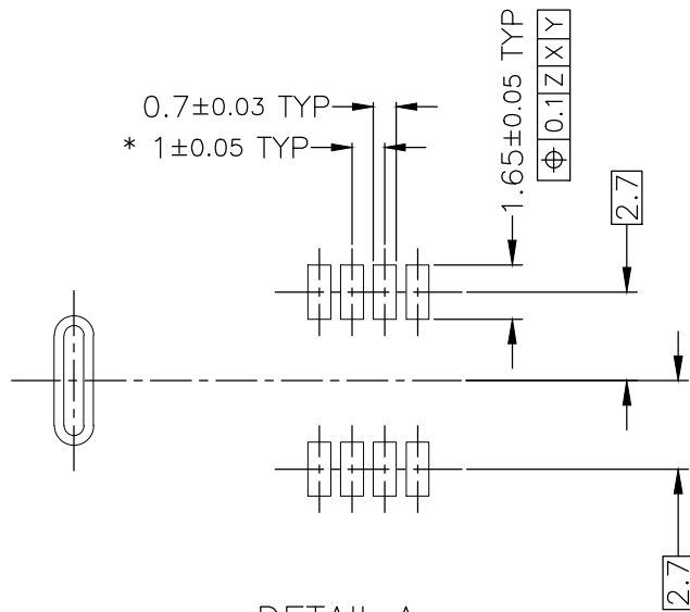
DETAIL A (4:1)
