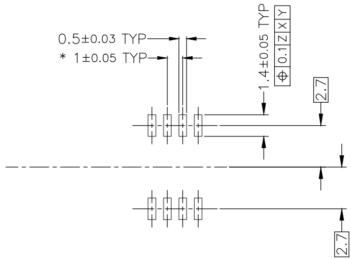
REFERENTIAL METAL MASK PAD OPENING (4:1)
