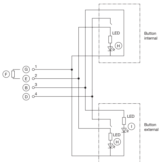
Wiring diagram 3
