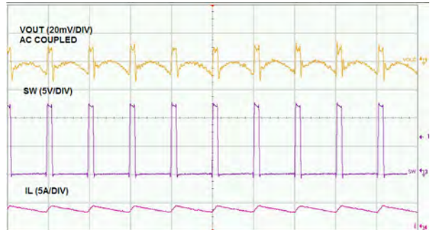
Time- 2µs/div Output Voltage Ripple
