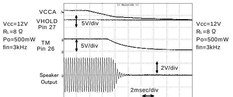
Fig. 16 Wave form on Instantaneous Power Interruption (2msec / div)
