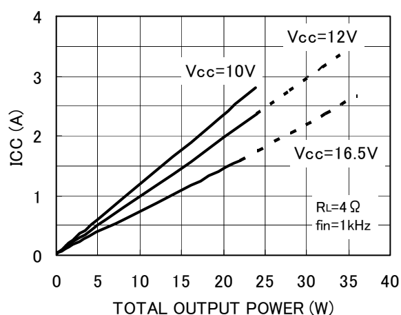
Fig. 27 Current consumption - Output power
