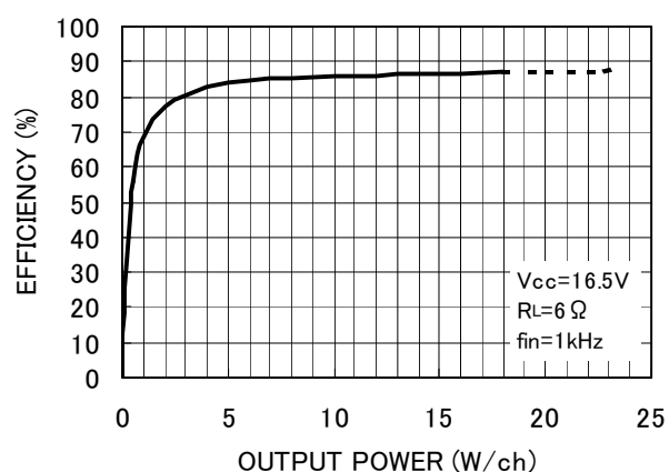
Fig. 21 Efficiency - Output power
