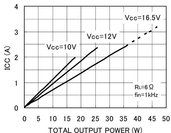
Fig. 22 Current consumption - Output power
