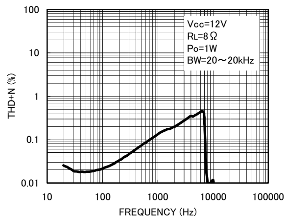
Fig. 2 THD+N — Frequency
