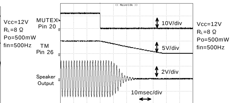
Fig. 14 Wave form when Activating Soft-mute
