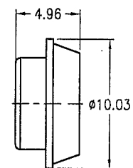
BRAID CLAMP
