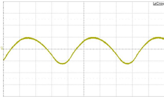
Fig. 15: Input reflected ripple current, i_c (1 A/div.), measured at input terminals at full rated load current and V_{in} = 48 V. Refer to Fig. 14 for test setup. Time scale: 2 \mu s/div.
