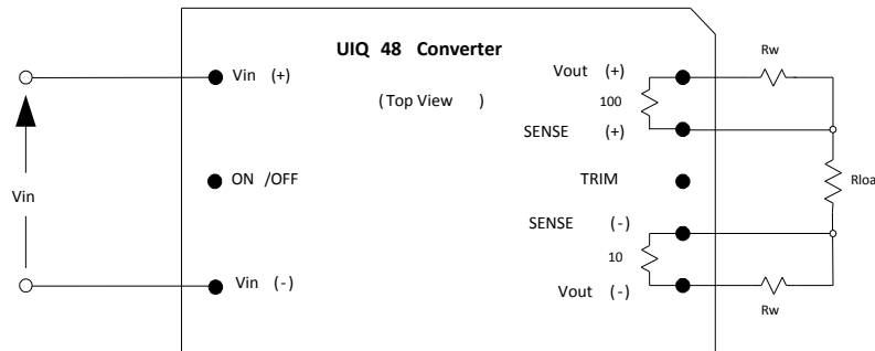
Fig. B: Remote sense circuit configuration.
