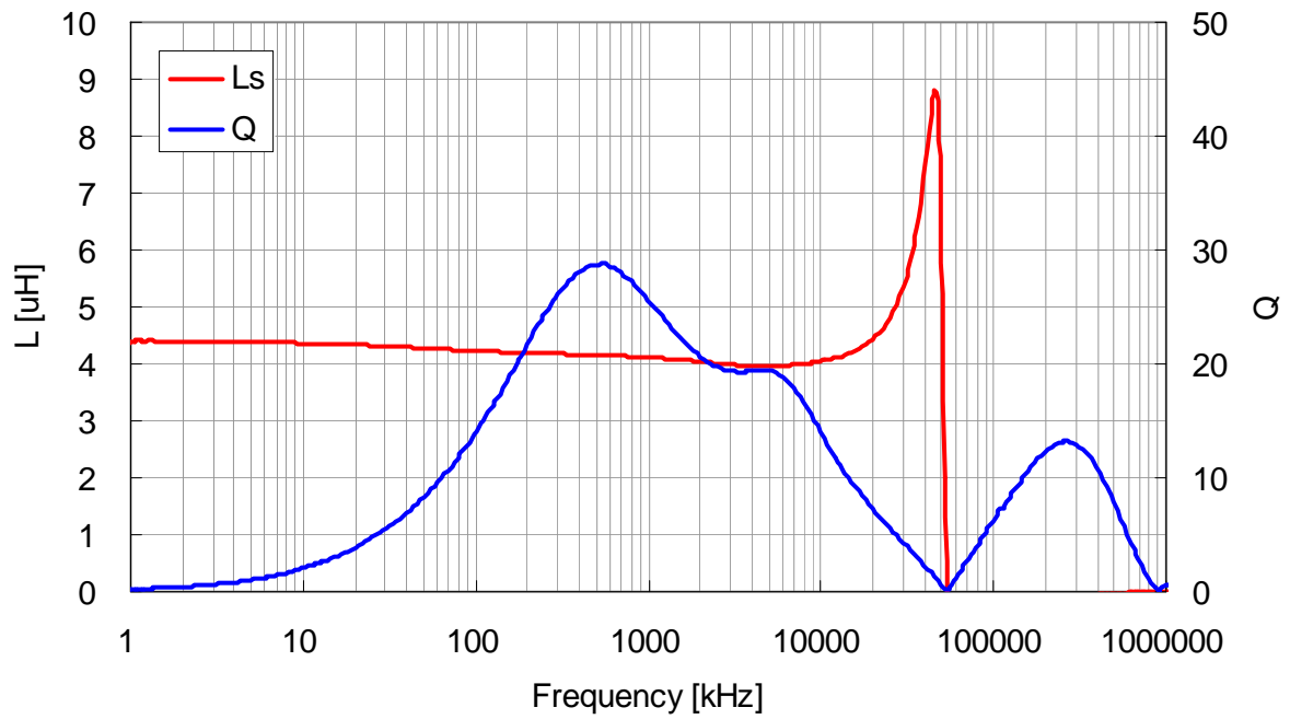
VLS3012T-4R7M1R0
