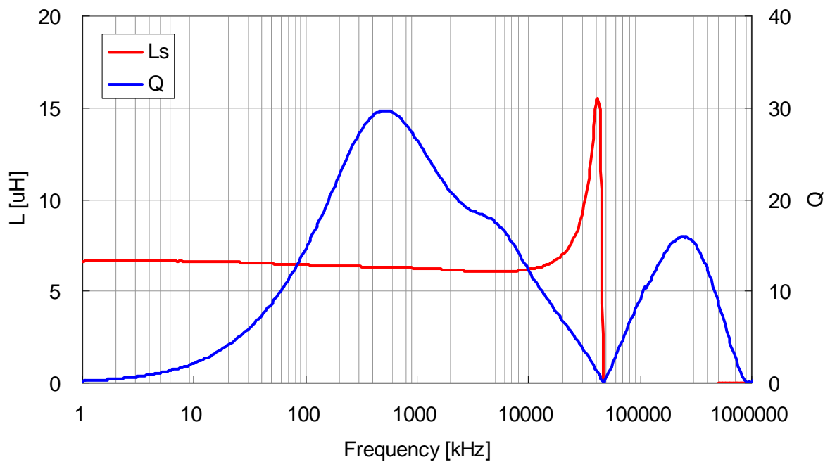
VLS3012T-6R8MR90
