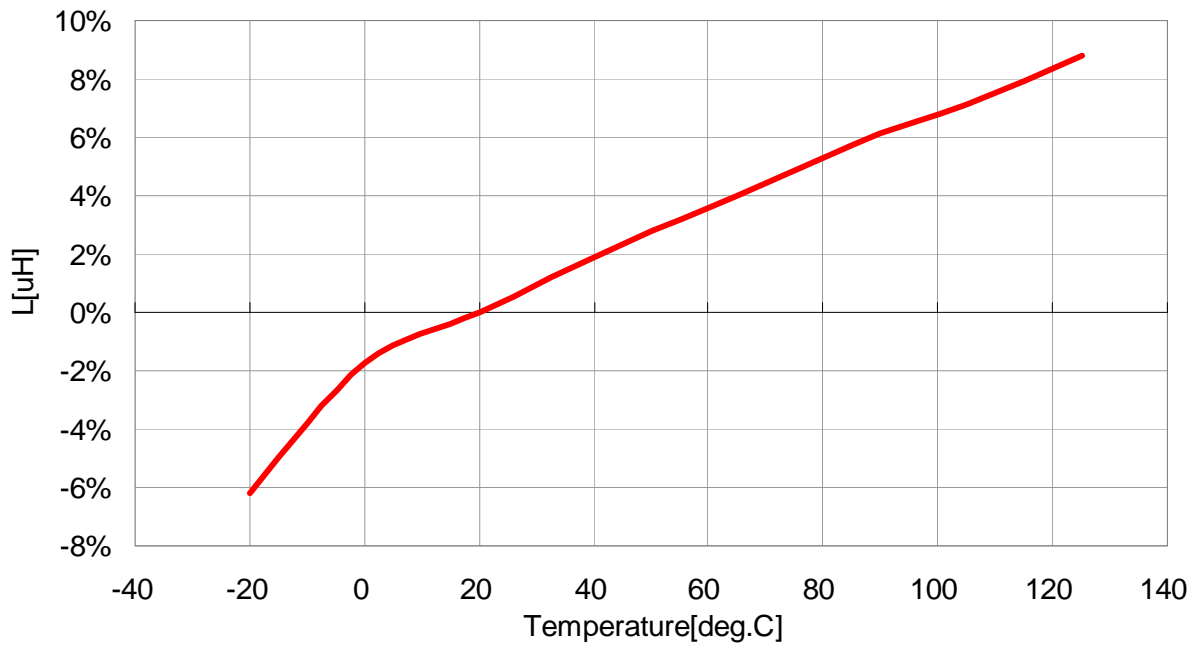
VLS3012T-4R7M1R0
