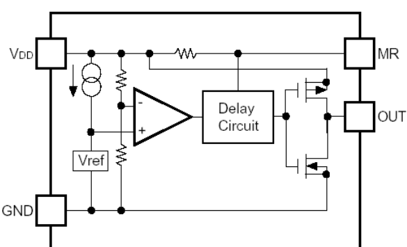
RP300xxxxC (CMOS Output)
