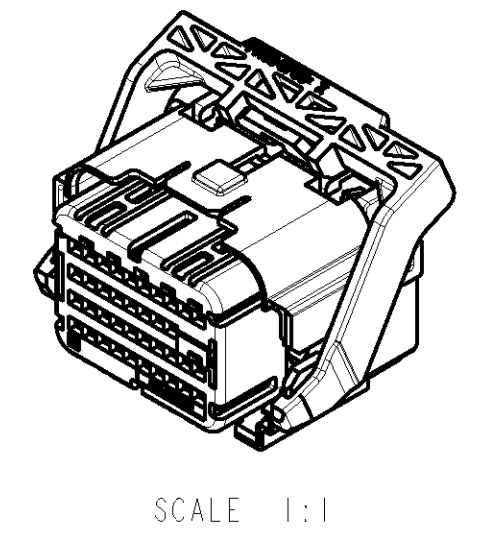
KEYING OPTION "G" SHOWN SEE SHEET 2 FOR BILL OF MATERIALS AND SHEET 3, 4 AND 5 FOR PIN-OUT CHARTS
