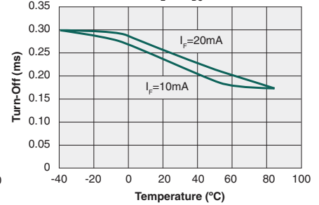
Typical Turn-Off vs. Temperature ( I_L=1\text{A}_{DC} )
