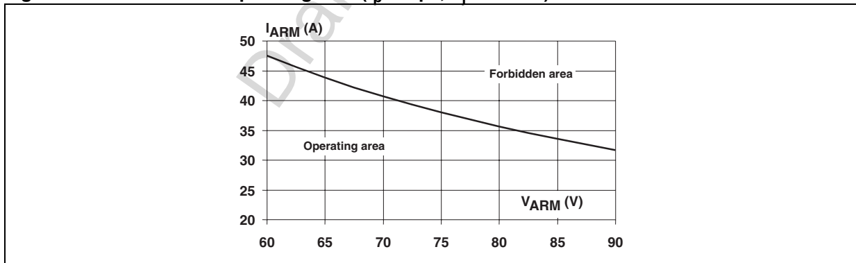
Figure 12. Reverse safe operating area ( t_p < 1 \mu s , T_i > 150 °C)
