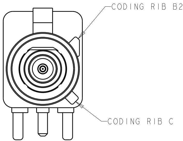
DETAIL H
