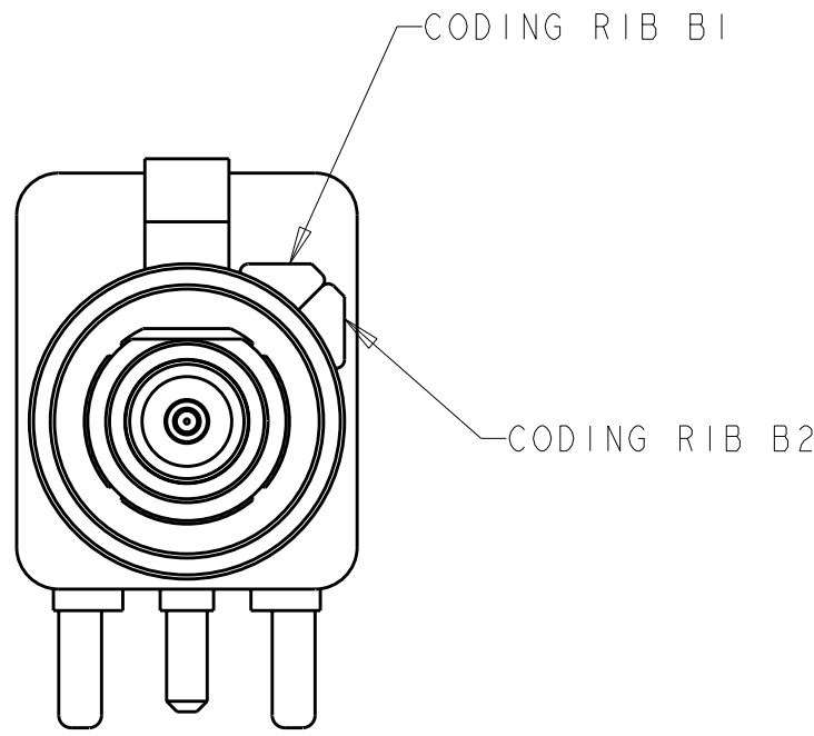
DETAIL E
