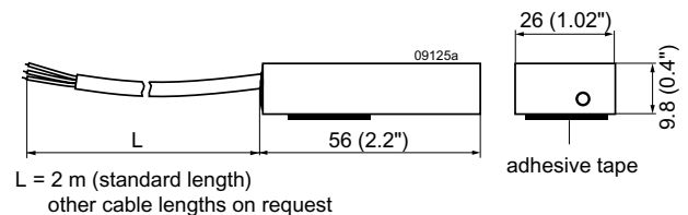
Fig. 6 S-KSMH temperature sensor.
