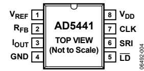
Figure 6. 8-Lead MSOP Pin Configuration
