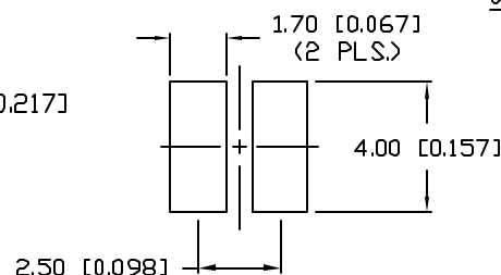
RECOMMENDED SOLDER PAD LAYOUT
