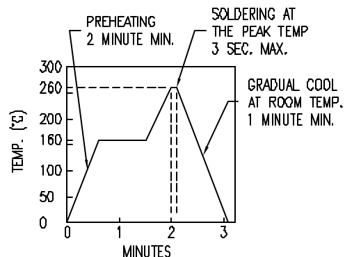
REFLOW PROFILE
