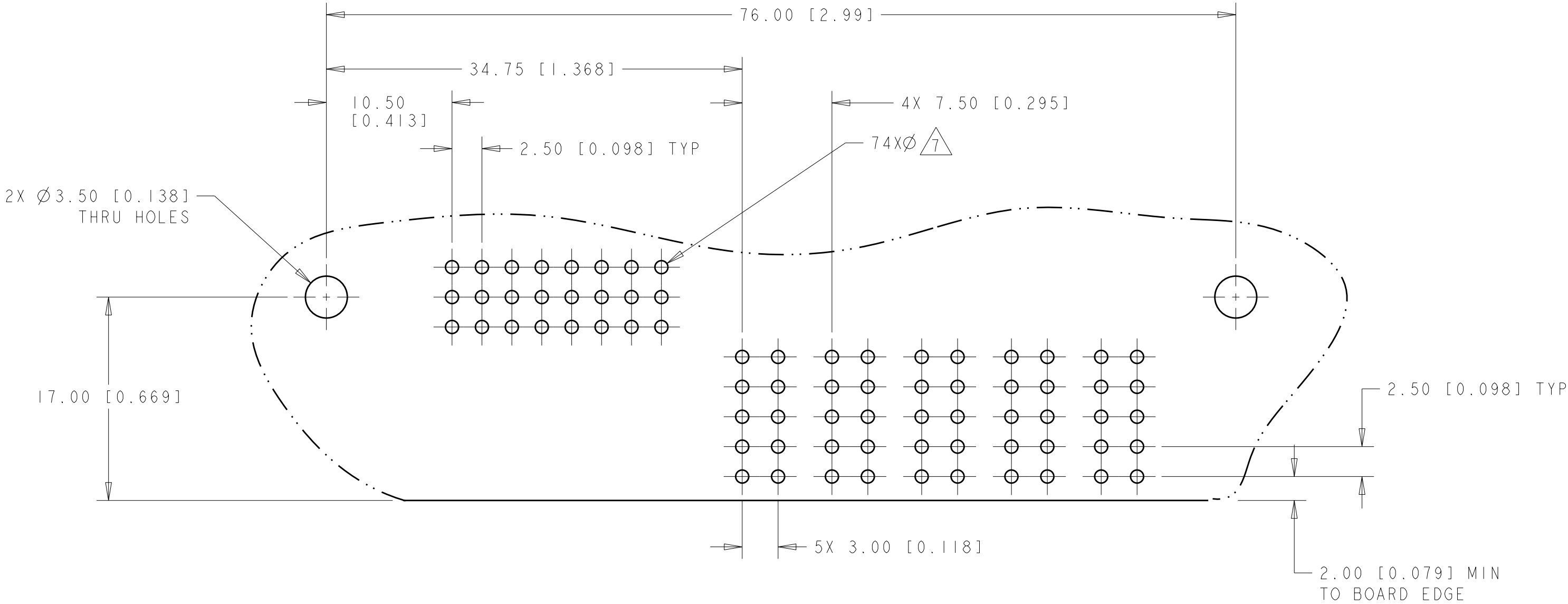
PRINTED CIRCUIT LAYOUT (AS VIEW FROM CONNECTOR SIDE)
