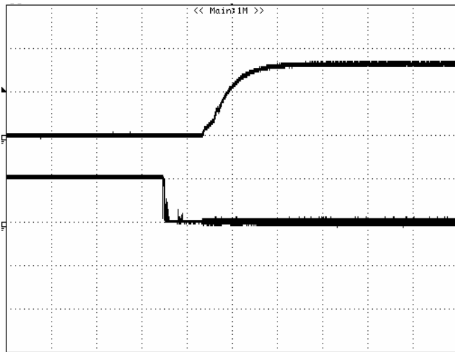
Figure 4: Turn-on transient at full rated load current (resistive load) (2 ms/div). V_{in}=48V . Top Trace: V_{out} , 2V/div; Bottom Trace: ON/OFF input, 5V/div
