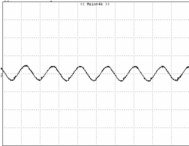
Figure 11: Input Terminal Ripple Current, i_c , at full rated output current and nominal input voltage with 12\mu\text{H} source impedance and 33\mu\text{F} electrolytic capacitor (100 mA/div, 2 us/div).
