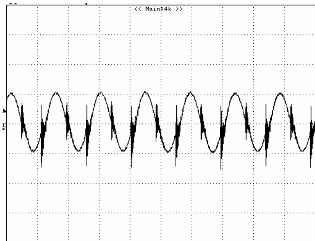
Figure 14: Output voltage ripple at nominal input voltage and rated load current ( I_o=25A ) (20 mV/div, 2 μs/div) Load capacitance: 1 μF ceramic capacitor and 10 μF tantalum capacitor. Bandwidth: 20 MHz. Scope measurements should be made using a BNC cable (length shorter than 20 inches). Position the load between 51 mm to 76 mm (2 inches to 3 inches) from the module.
