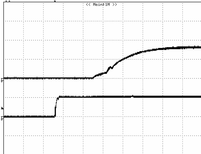
Figure 6: Turn-on transient at full rated load current (resistive load) (2 ms/div). V_{in}=48V . Top Trace: V_{out} , 2V/div; Bottom Trace: ON/OFF input, 5V/div
