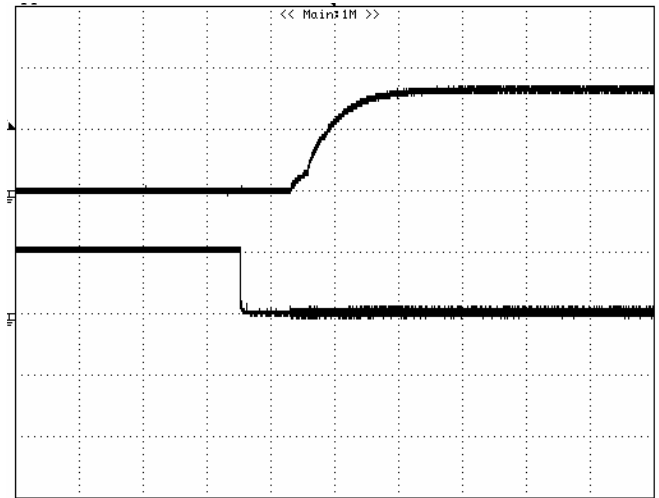
Figure 5: Turn-on transient at zero load current (2 ms/div). V_{in}=48V . Top Trace: V_{out} , 2V/div; Bottom Trace: ON/OFF input, 5V/div
