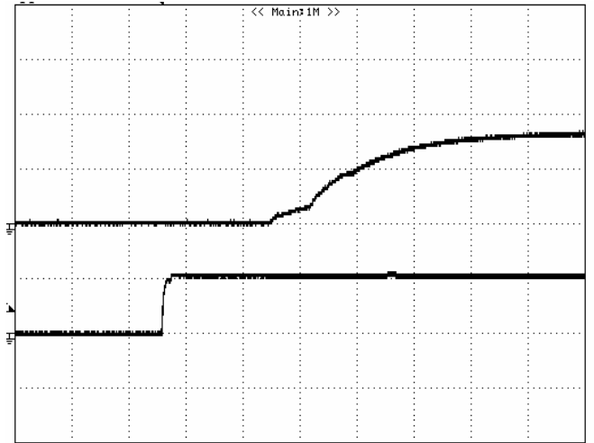
Figure 7: Turn-on transient at zero load current (2 ms/div). V_{in}=48V . Top Trace: V_{out} , 2V/div; Bottom Trace: ON/OFF input, 5V/div
