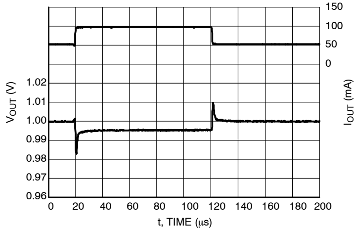
Figure 67. Load Transients, 1.0 V Version, I OUT = 50 - 100 mA, t R = t F = 0.5 μs, V IN = 2.0 V, AE = 0 V
