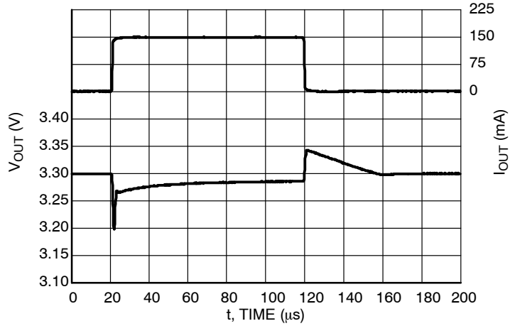
Figure 66. Load Transients, 3.3 V Version, I OUT = 1 - 150 mA, t R = t F = 0.5 μs, V IN = 4.3 V, AE = V IN V
