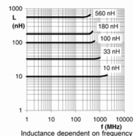
Inductance dependent on frequency
