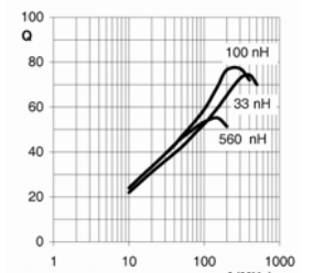
Typical Q - shape dependent on frequency
