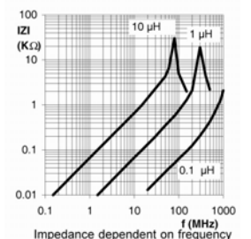
Impedance dependent on frequency
