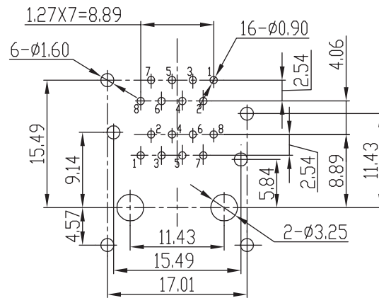
PCB LAYOUT - COMPONENT VIEW THICKNESS = 1,6 MM
