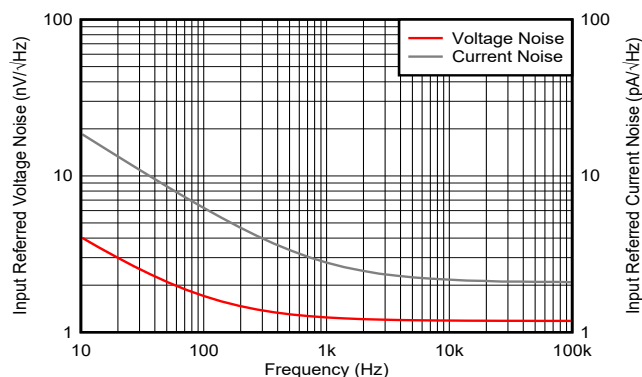
Voltage and Current Noise vs Frequency
