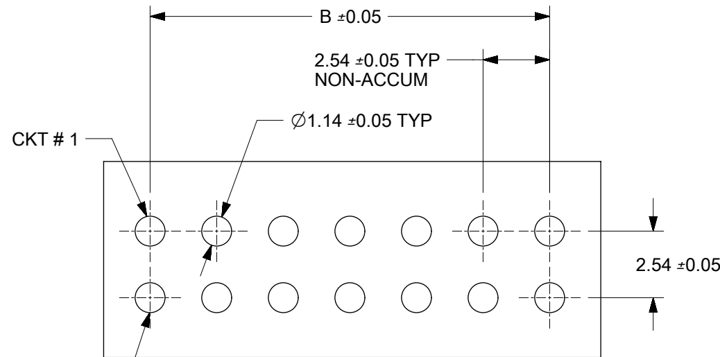
RECOMMENDED PCB HOLE LAYOUT
