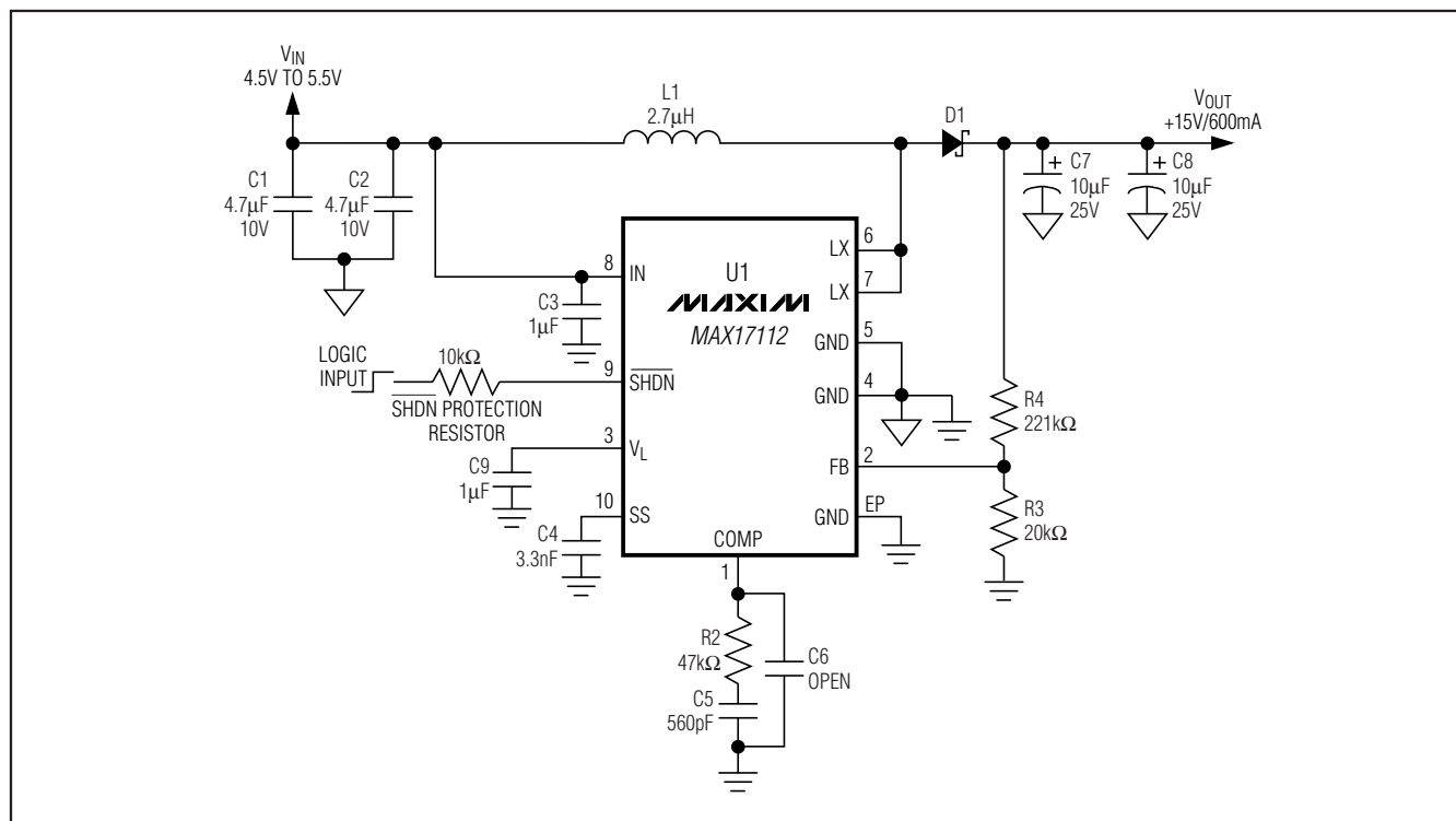
Figure 3. Application Circuit Using Logic Input at \overline{\text{SHDN}}
