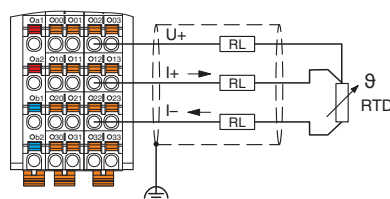
Connection example: 3-wire connection
