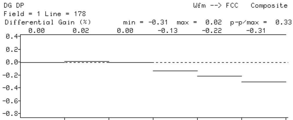
Figure 7. Differential Gain
