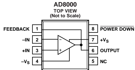
Figure 1. 8-Lead AD8000, 3 mm x 3 mm LFCSP (CP-8-13)
