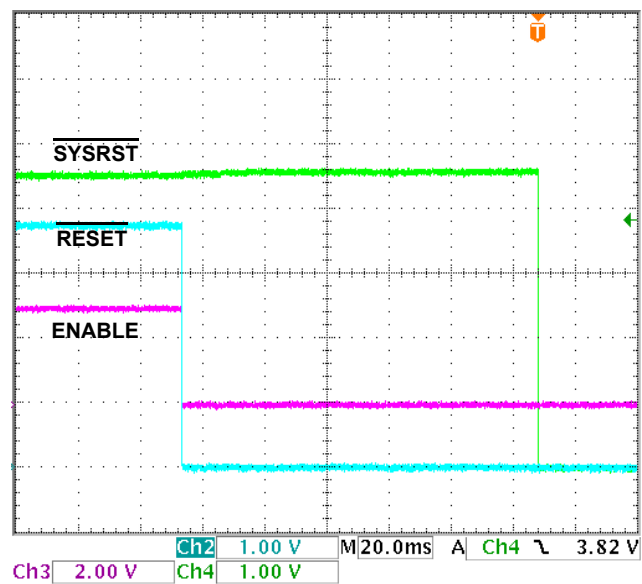
FIGURE 20. ENABLE LOW TO RESET AND SYSRST LOW
