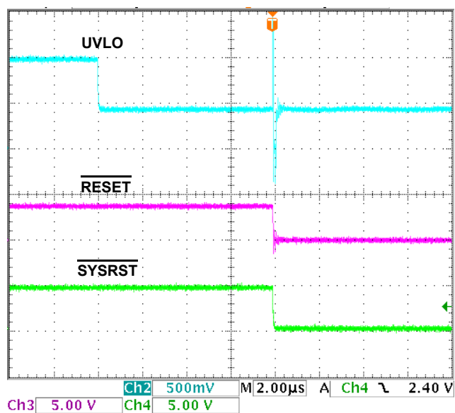
FIGURE 21. UVLO INVALID TO RESET AND SYSRST LOW
