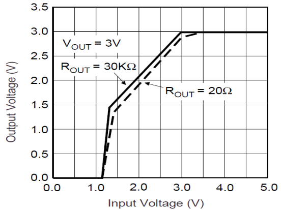
Figure 20. Dropout Characteristics
