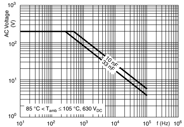
RMS voltage as a function of frequency
