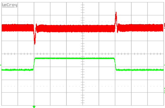
Figure 8. Output voltage response to load current step (3.5 A–5.25 A–3.5 A) at V_{in} = 48\text{ V} . Top trace: output voltage (100 mV/div.). Bottom trace: load current (2 A/div.). Current slew rate: 0.1 A/ \mu\text{s} . C_o = 1\text{ }\mu\text{F} ceramic + 10 \mu\text{F} tantalum. Time scale: 0.2ms/div.
