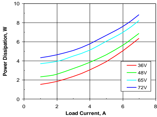
Figure 4. Power dissipation vs. load current and input voltage for SSQE48T07120 converter mounted vertically with air flowing from pin 1 to pin 3 at a rate of 300 LFM (1.5 m/s) and T_a = 25\text{ }^\circ\text{C} .
