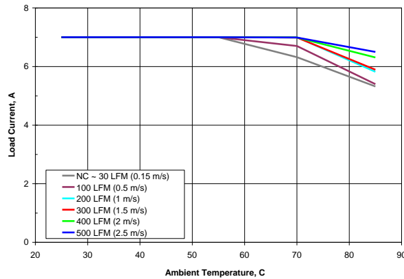
Figure 1. Available load current vs. ambient air temperature and airflow rates for SSQE48T07120 converter mounted vertically with air flowing from pin 1 to pin 3, V_{in} = 48\text{ V} . Note: NC – Natural convection
