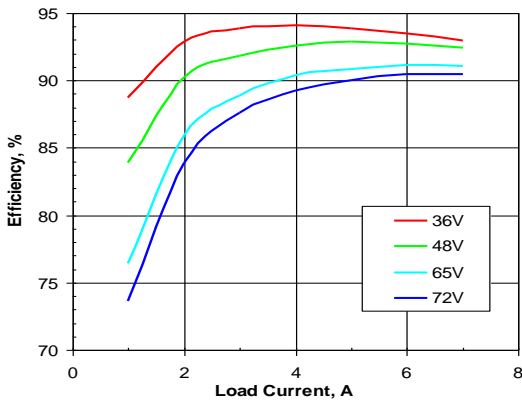
Figure 2. Efficiency vs. load current and input voltage for SSQE48T07120 converter mounted vertically with air flowing from pin 1 to pin 3 at a rate of 300 LFM (1.5 m/s) and T_a = 25\text{ }^\circ\text{C} .
