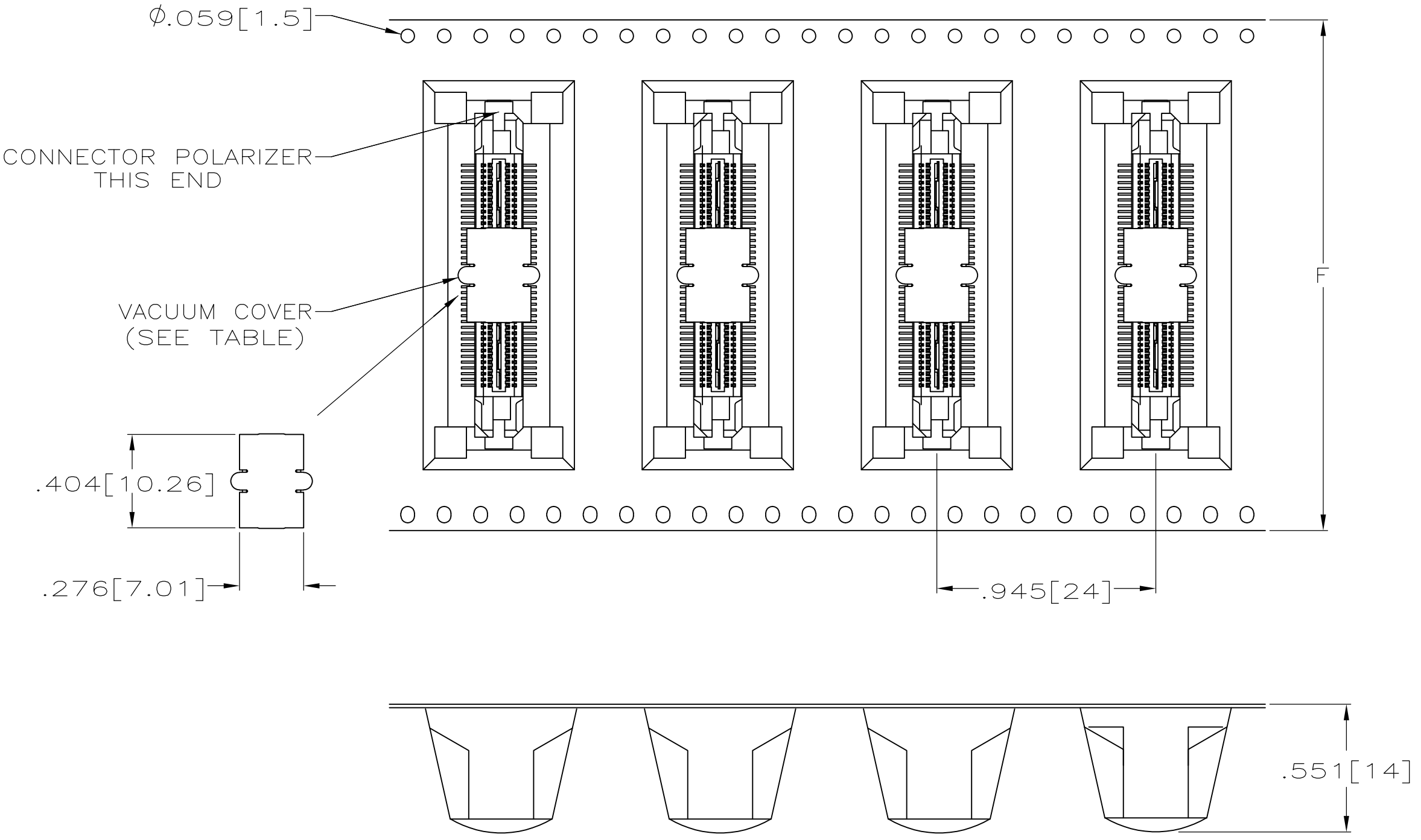
PACKAGING DETAIL A SCALE 2:1 DIMENSIONS ARE FOR REFERENCE
