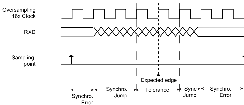
Figure 34-11. Bit Resynchronization
