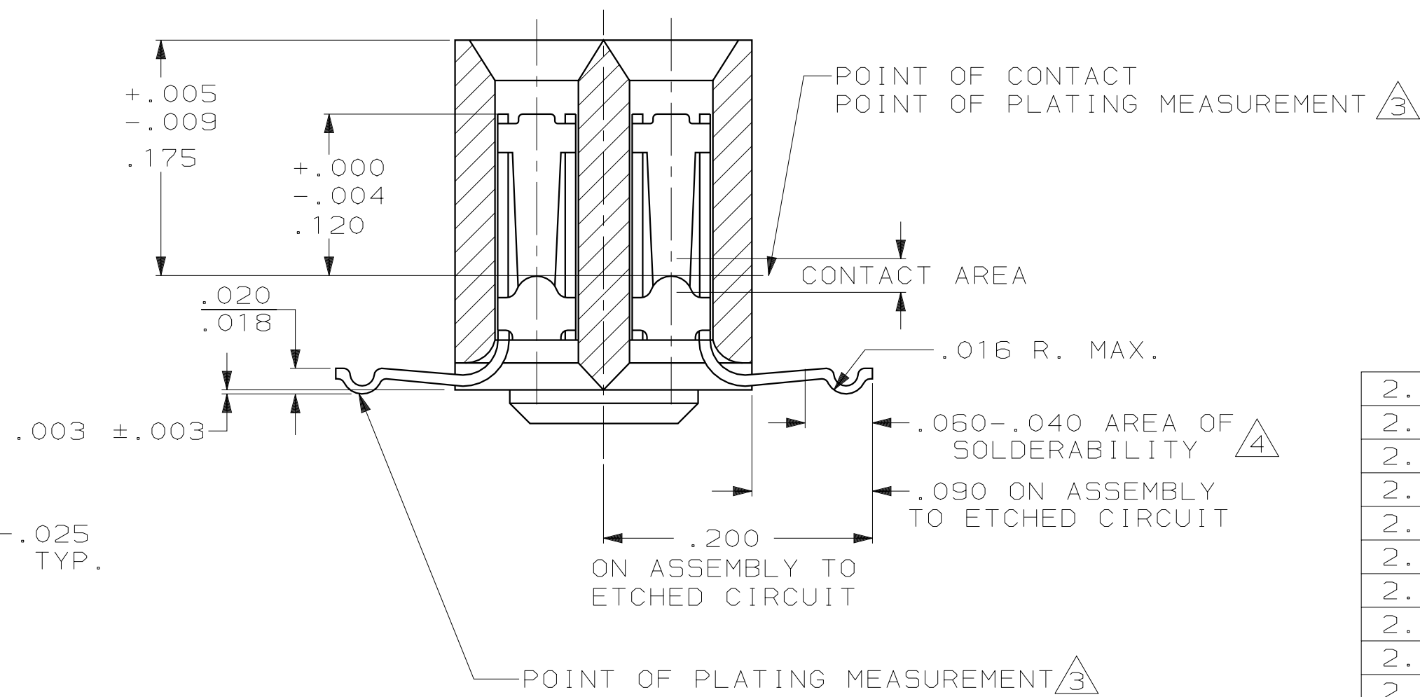
SECTION Z-Z
