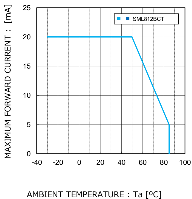
Fig.4 Derating
