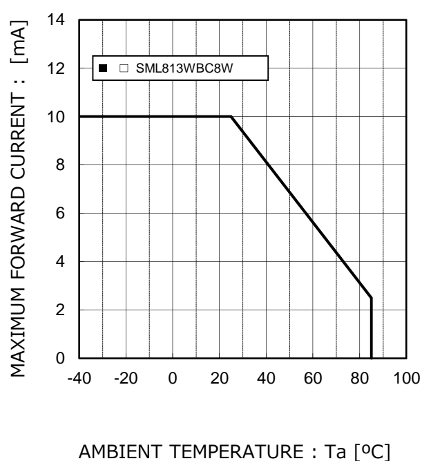
Fig.4 Derating
