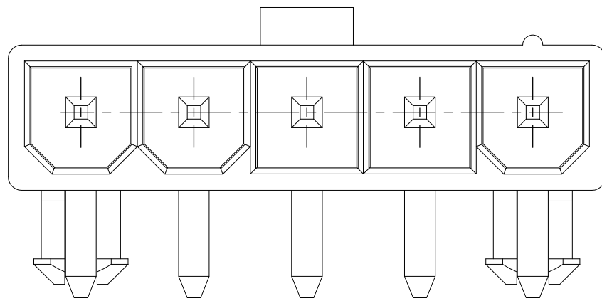
2029154-5 MATING FACE
