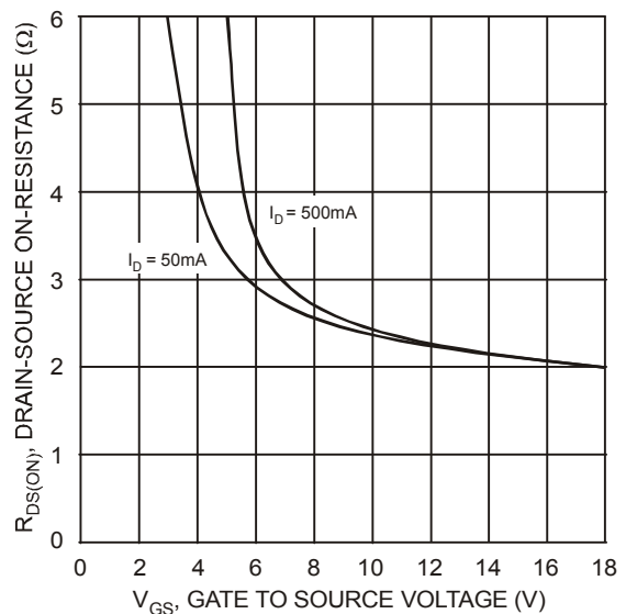
Fig. 11 On-Resistance vs. Gate-Source Voltage (2N7002)
