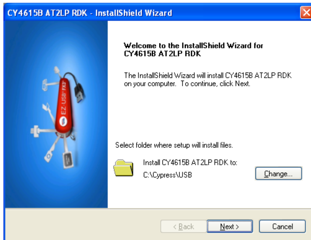
Figure 2-2. InstallShield Wizard
