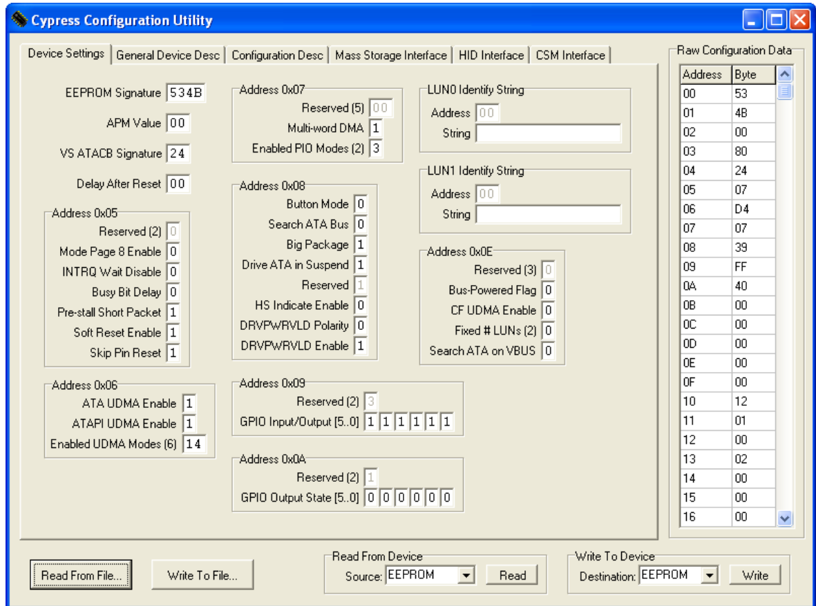
Figure 4-1. Configuration Utility
