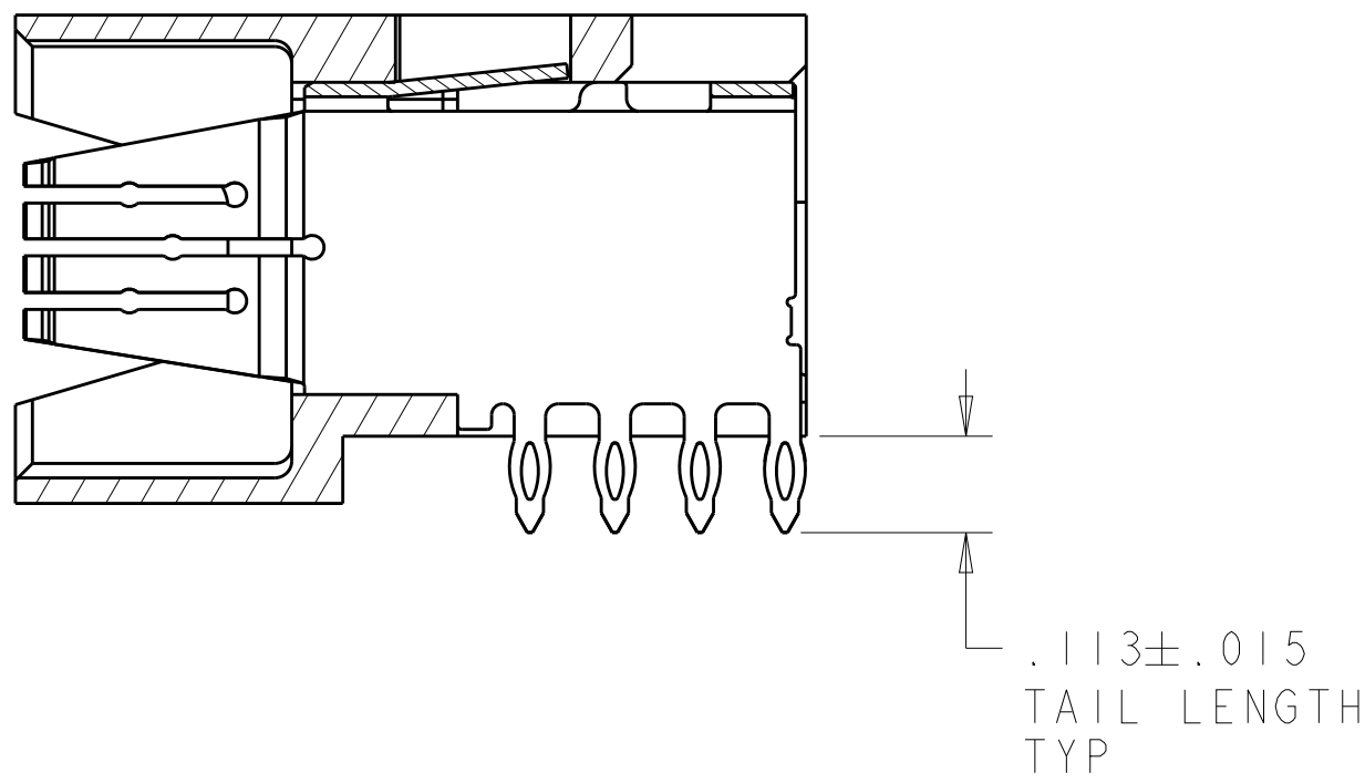
SECTION Z-Z
