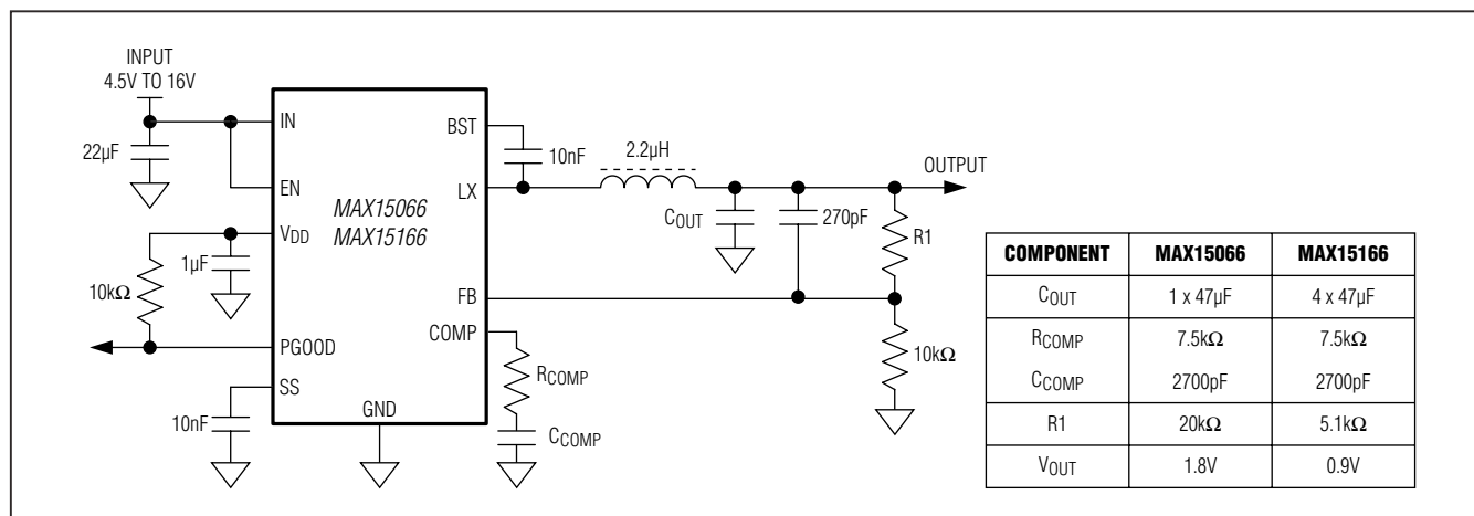
Figure 1. Reference Circuit
