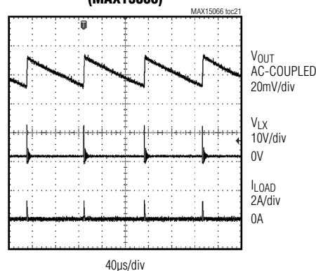
SKIP MODE WAVEFORM (MAX15066)
