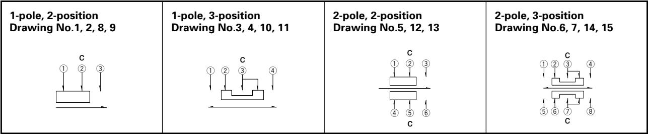
■ Circuit Diagram (Viewed from Direction A)
