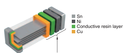
Soft termination
