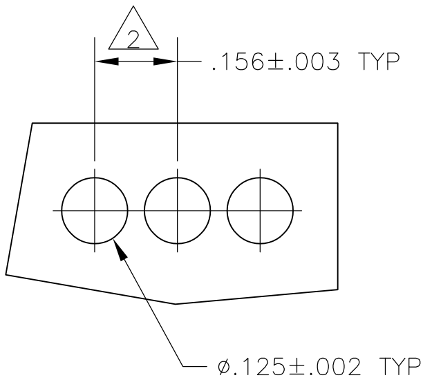
RECOMMENDED BOARD MOUNTING (RECOMMENDED BOARD THICKNESS: .055-.070)
