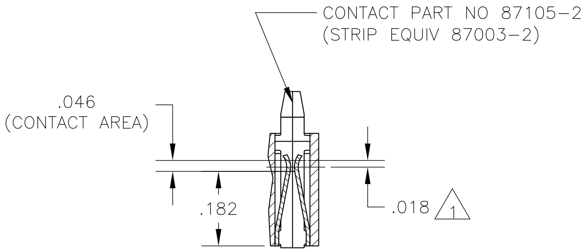
SECTION X-X
