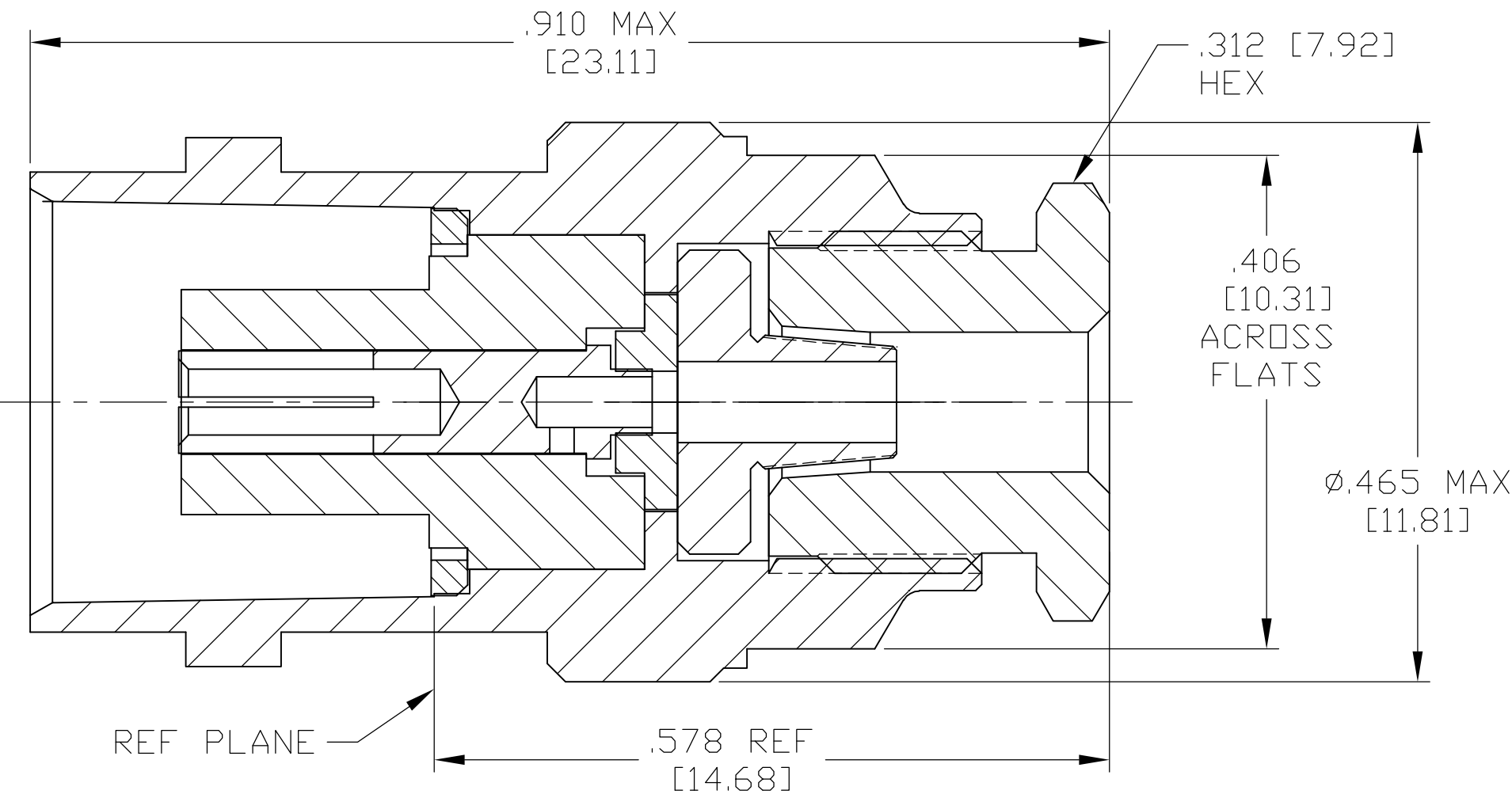
ASSEMBLED VIEW
