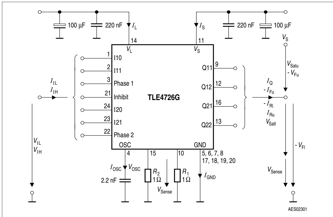
Figure 3 Test Circuit
