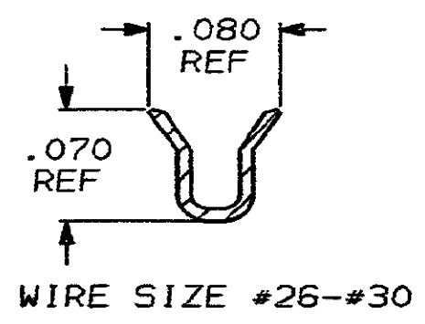
SECTION C-C
