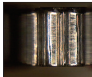
Unplated Crimper Surface after 60,000 Terminations. Note Significant buildup of material.
