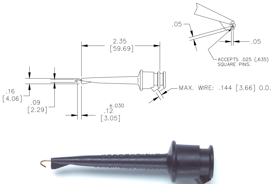
Model 4555 Do-It-Yourself Minigrabber Test Clip
